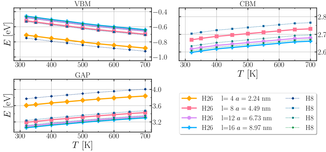
Figure D.13. Energies of band edges and gap for \text{CsPbCl}_3 circular quantum wire at different temperatures for several selected sizes, where l is the diameter of the circular base of the wire, and VBM (CBM) are valence band maximum (conduction band minimum).
