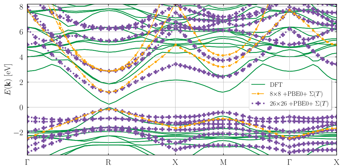
Figure 3.9. Band structure of the cubic phase of \text{CsPbI}_3 calculated using standard and extended \mathbf{k} \cdot \mathbf{p} Hamiltonian parametrized using band energies obtained using hybrid PBE0 functional and self-energy correction \Sigma(T) at T=300 K that stems from the phonon-induced renormalization of band energies. DFT results obtained with PBE functional are also given for comparison.
