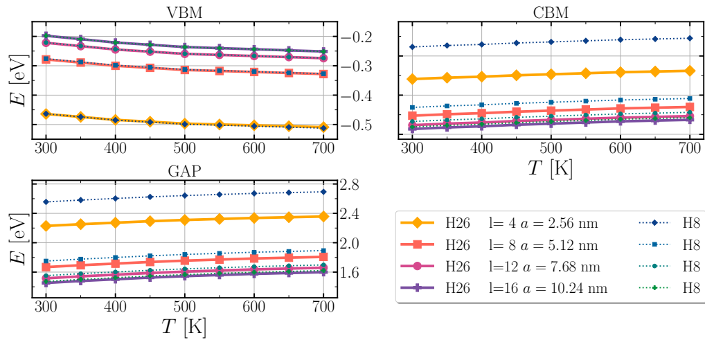
Figure D.9. Energies of band edges and gap for \text{CsPbI}_3 spherical quantum dots at different temperatures for several selected sizes, where l is the length of one edge of the cube, and VBM (CBM) are valence band maximum (conduction band minimum).
