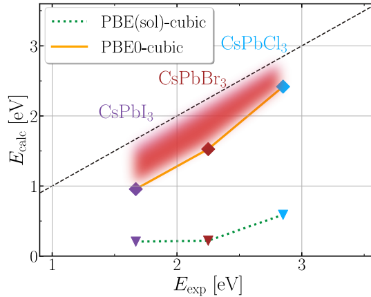
Figure 4.1. Comparison of experimental and theoretical results for the electronic gap for \text{CsPbX}_3 ( X = \text{Cl}, \text{Br} or \text{I} ) calculated without taking temperature effects into account. The line x = y represents the experimental results for lowest temperature of the cubic structure. The symbols denote calculated values for the cubic structure using the PBE (PBEsol) functional for \text{CsPbI}_3 ( \text{CsPbCl}_3 and \text{CsPbBr}_3 ) (inverted triangles) and PBE0 functional modified to satisfy the Koopmans condition (diamonds).
