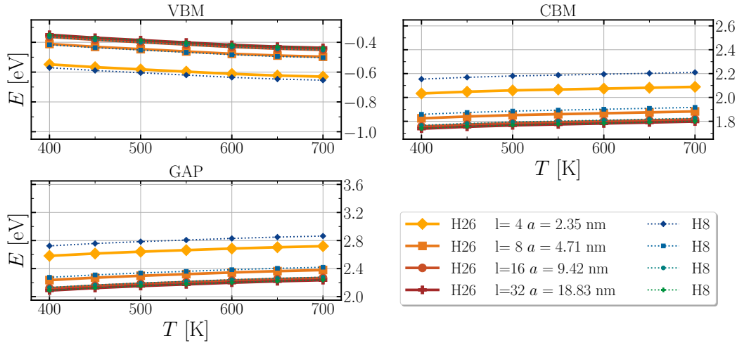
Figure 5.17. Energies of band edges and gap for \text{CsPbBr}_3 squared quantum wires at different temperatures for several selected sizes, where l is the length of the edge of the square base of the wire, and VBM (CBM) are valence band maximum (conduction band minimum).
