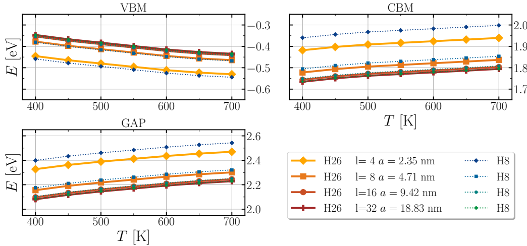
Figure D.14. Energies of band edges and gap for \text{CsPbBr}_3 circular quantum wire at different temperatures for several selected sizes, where l is the diameter of the circular base of the wire, and VBM (CBM) are valence band maximum (conduction band minimum).
