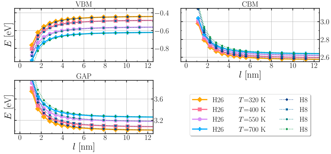
Figure D.10. Energies of band edges and gap for CsPbCl 3 quantum wires of different cross section sizes at several selected temperatures, where l is the diameter of the circular base of the wire, and VBM (CBM) are valence band maximum (conduction band minimum).
