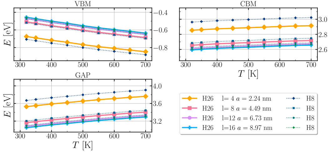
Figure 5.16. Energies of band edges and gap for \text{CsPbCl}_3 squared quantum wires at different temperatures for several selected sizes, where l is the length of the edge of the square base of the wire, and VBM (CBM) are valence band maximum (conduction band minimum).
