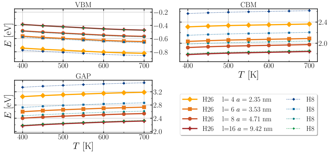
Figure D.8. Energies of band edges and gap for \text{CsPbBr}_3 spherical quantum dots at different temperatures for several selected sizes, where l is the length of one edge of the cube, and VBM (CBM) are valence band maximum (conduction band minimum).
